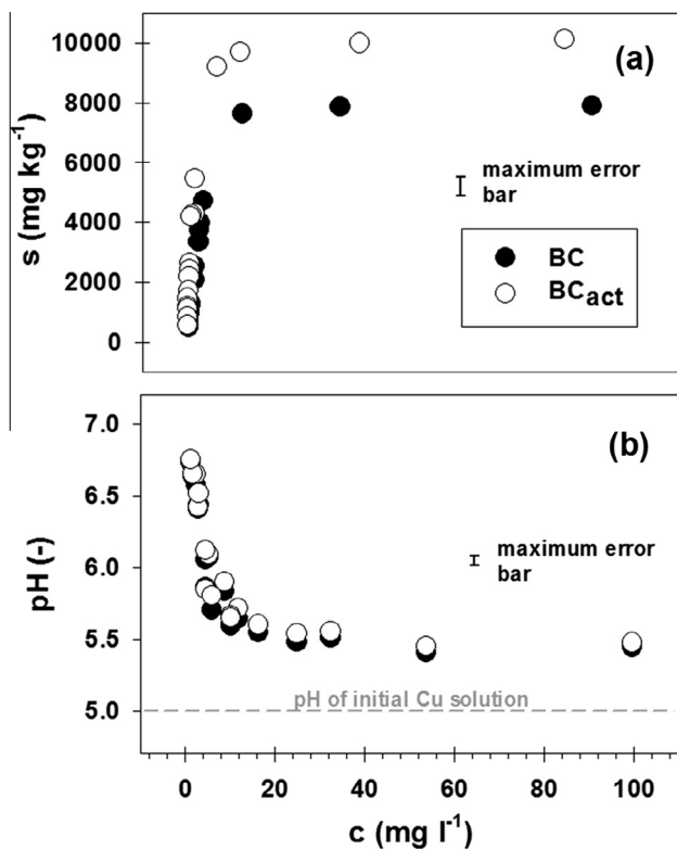
Figure 6 Sorption isotherms (a) and pH changes (b) during Cu sorption from synthetic solution for biochar (BC) and activated biochar (BC act ).
