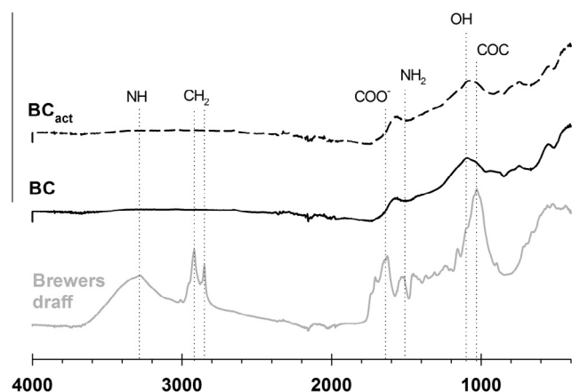
Figure 4 FTIR spectrum of (i) brewers draff before pyrolysis; (ii) biochar (BC), and (iii) activated biochar (BC act ).
